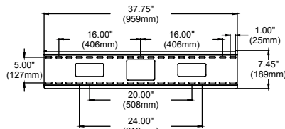
WALL PLATE
