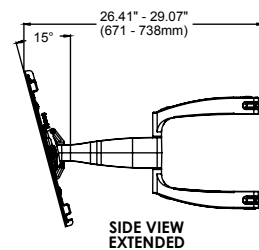
SIDE VIEW EXTENDED
