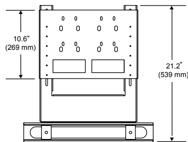
MSA-101
