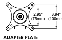
ADAPTER PLATE
