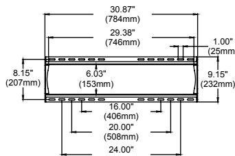
WALL PLATE
