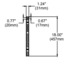
VERTICAL ADAPTER
