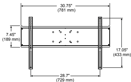
ADAPTER BRACKET DETAIL (PLCK-UNL ONLY)
