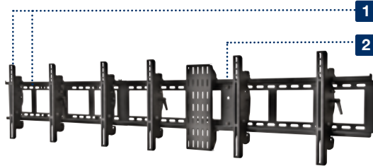
Configuration Shown: DS-VL-H048 and DS-VL-H036 and ACC-DSV329 with accessory DS-ACC-LDCM
