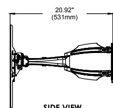
SIDE VIEW EXTENDED
