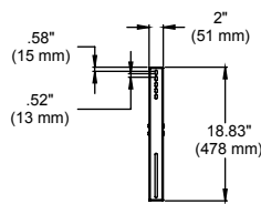
FRONT OF SCREEN ADAPTER
