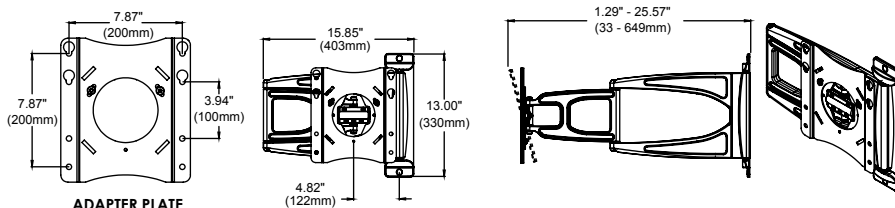
ADAPTER PLATE
