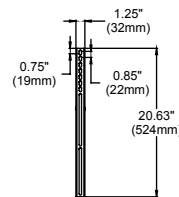
VERTICAL BRACKET
