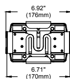
FRONT VIEW RETRACTED
