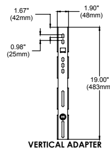
VERTICAL ADAPTER
