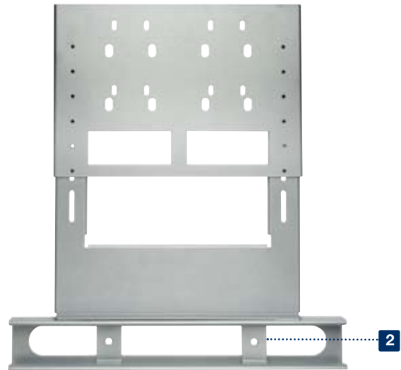
MSA-101
