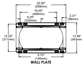
WALL PLATE
