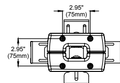
REAR MOUNTING HOLES
