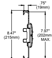
SIDE VIEW EXTENDED
