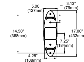
WALL PLATE
