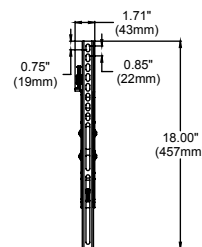
VERTICAL ADAPTER
