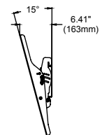
SIDE VIEW 15° TILT
