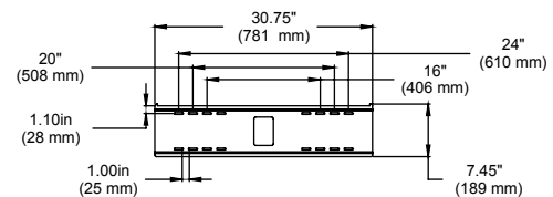
WALL PLATE
