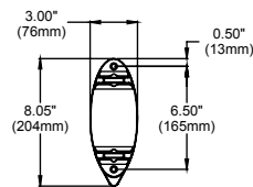
WALL PLATE
