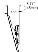
SIDE VIEW 15° TILT
