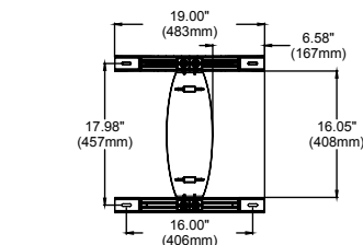
WALL PLATE
