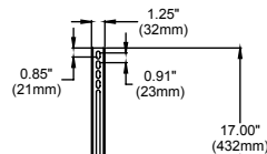
VERTICAL ADAPTER
