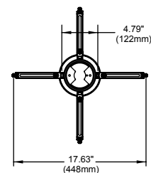
ADAPTER PLATE
