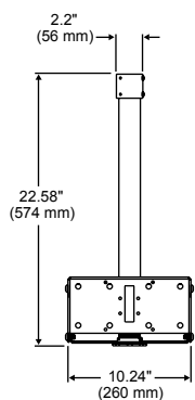
PLCK-1, PLCK-UNL (without adapter plate)
