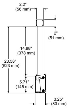
PLCK-1, PLCK-UNL (without adapter plate)
