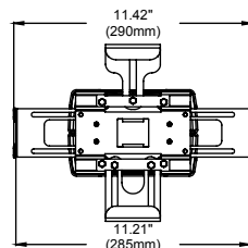
FRONT VIEW EXTENDED
