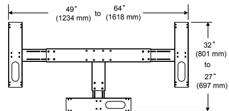
MSA-301
