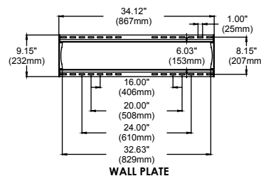
WALL PLATE
